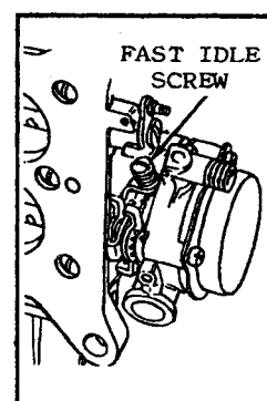
FIG. 5 FAST IDLE ADJUSTMENT
