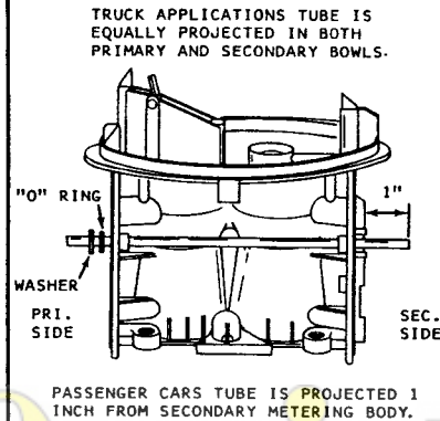
BALANCE TUBE POSITION FIG. 5
