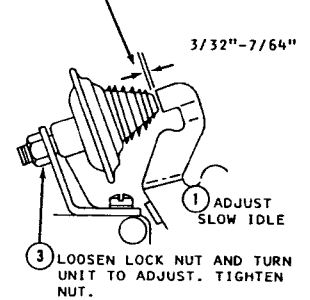
SLOW CLOSING THROTTLE ADJ. FIG. 14
