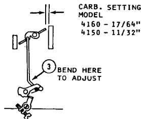
UNLOADER ADJUSTMENT FIG. 9
