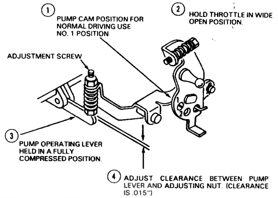
PUMP ADJUSTMENT
