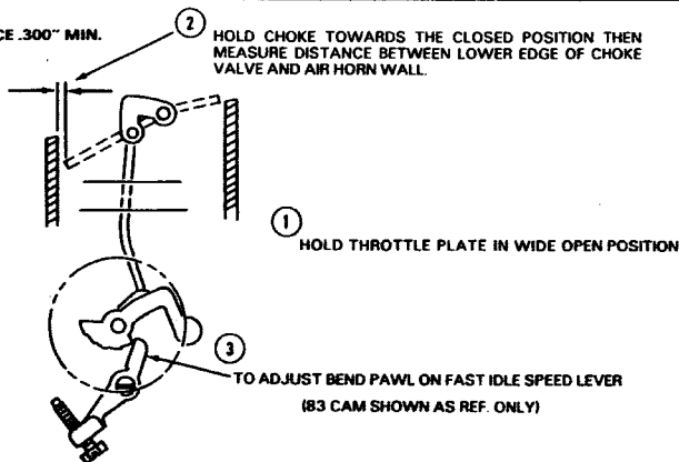
UNLOADER ADJUSTMENT
