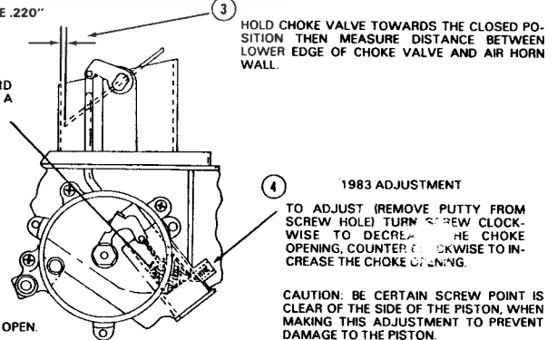
(ALSO SEE FIG. 9) CHOKE PLATE PULLDOWN ADJUSTMENT
