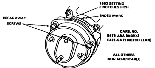
AUTOMATIC CHOKE SETTING
